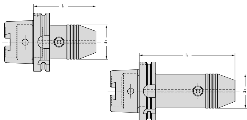
Short drill chucks HSK Form A with coolant feed
